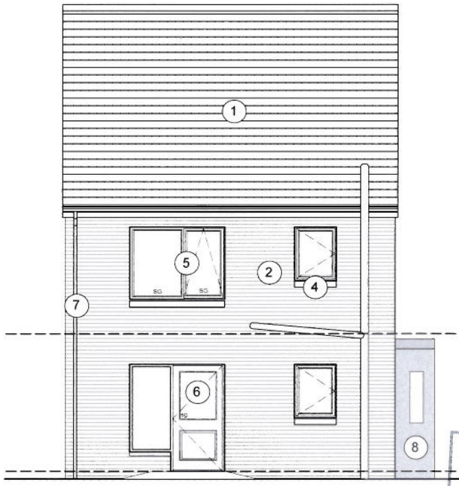
HOUSE TYPE - L1 REAR ELEVATION
