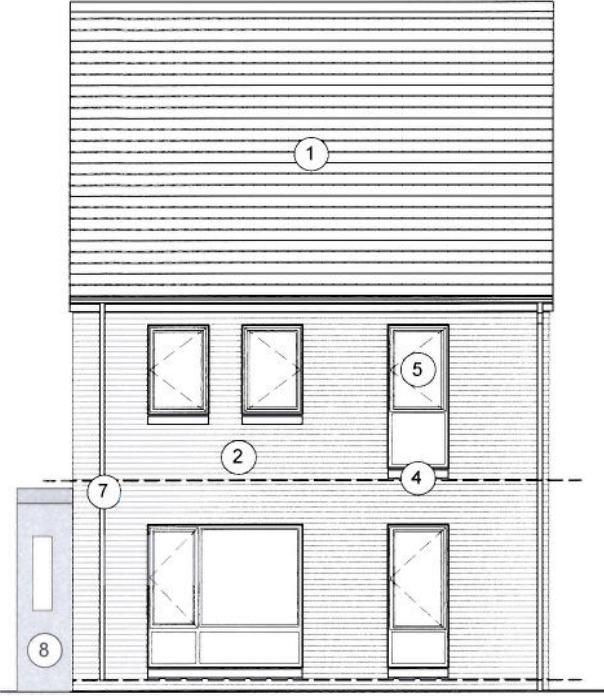
HOUSE TYPE - L1 FRONT ELEVATION
