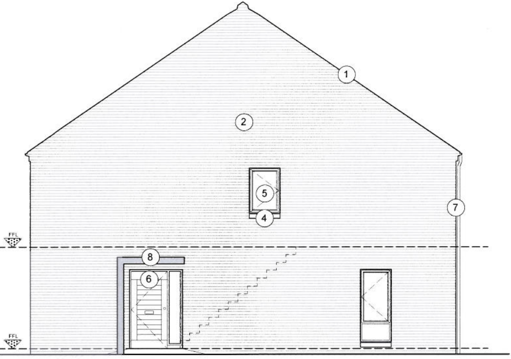
HOUSE TYPE - L1 SIDE ELEVATION
